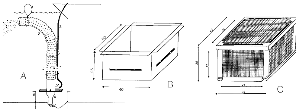
Fig. 1. Schematic diagram of an airlift (A) sucking out bottom contents from inside an aluminum digging frame (B) (1 = buoy, 2 = flexible hose, 3 = air hose, 4 = sucking tube, 5 = digging frame in situ) and an exclusion cage (C). All measurements in centimetres
